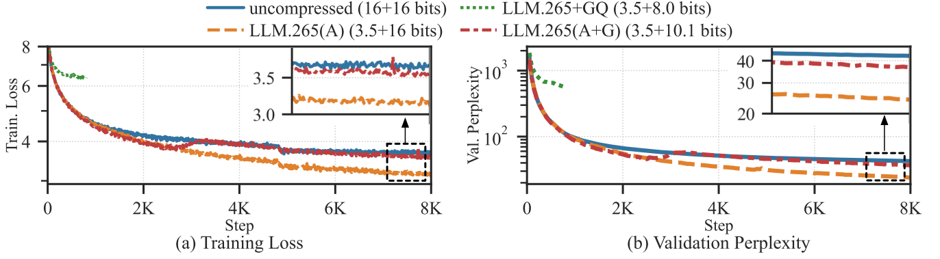
Figure 9: Training loss and validation perplexity of Pythia 1.4B using pipeline parallelism.
