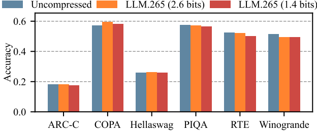
Figure 11: Evaluation results of trained Pythia 160M models on commonsense reasoning tasks.
