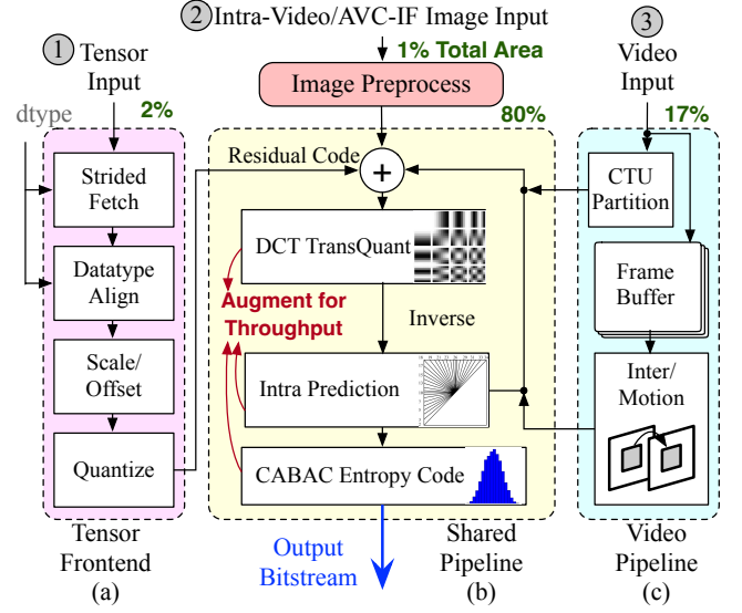
Figure 13: We modified the H.264 video codec to enable the encoding and decoding of tensors, images, and videos. The three-in-one encoder illustrated in this figure supports encoding tensors at a throughput of 100 Gbps and videos at 8K resolution and 60 fps.
