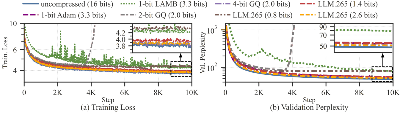
Figure 10: Training loss and validation perplexity of Pythia 160M using data parallelism.
