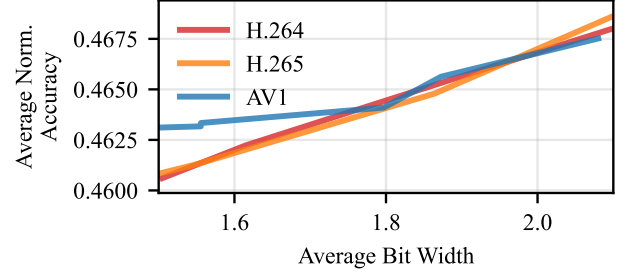
Figure 6: Comparison of the tensor compression information efficiency of the three most popular video codecs: H.264, H.265, and AV1. At a reasonable storage budget, the difference in information efficiency between all three codecs is so small that can be attributed to noise.
