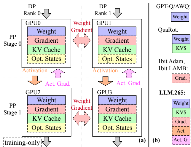
Figure 1: LLM.265: General-Purpose and Versatile Tensor Compression for LLM Training and Inference.
