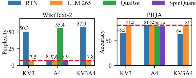
Figure 8: The comparison between RTN quantization, SpinQuant [48], QuaRot [4] and LLM.265 for compressing KV cache and activations of LLaMA-3-70B. "KV3" means compressing the KV cache to 3 bits (2.9 bits for LLM.265), while "A4" compresses activations to 4 bits (3.5 bits for LLM.265). Lower perplexity and higher accuracy indicate better compression quality.
