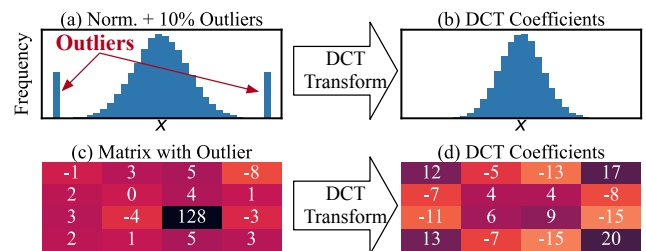
Figure 3: Transform coding mitigates encoding outliers by mapping them to all values within the block. The transition from (a) to (b) demonstrates how DCT removes outliers from a normal distribution containing outliers. (c) to (d) gives an example of an outlier with a value of 128 being mitigated.
