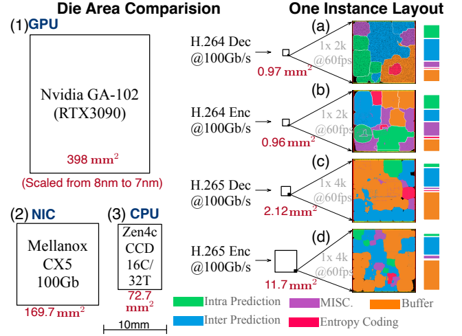
Figure 12: Comparison of the chip die area between GPU (1), CPU (3), NIC (2), and Video Codecs (a-d). Multiple instances of video encoders or decoders are combined to achieve a total throughput of 100Gb/s.
