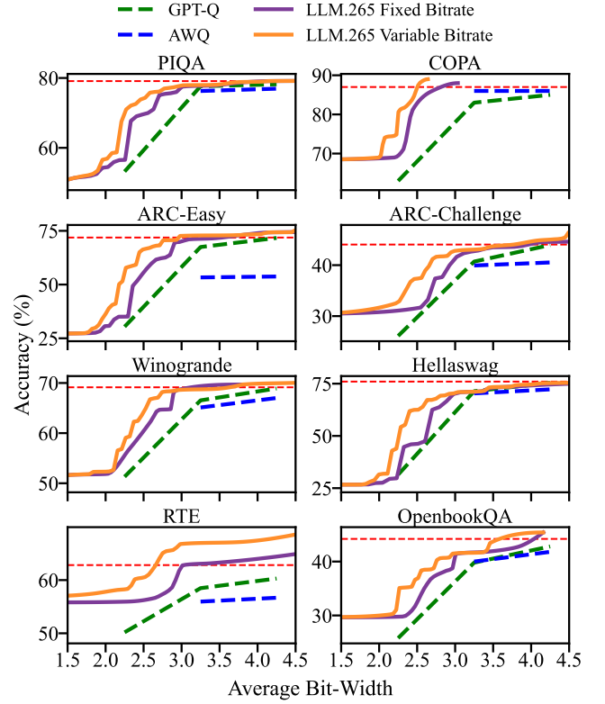
Figure 5: The trade-off between accuracy and average bit-width of different methods for compressing the LLaMA-2-7B model [78] on eight commonsense reasoning tasks. The red-dashed-line represents the BF16 uncompressed model accuracy.
