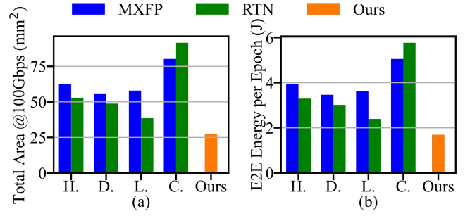
Figure 15: Comparing Three-in-one codec with existing solutions: (a) The total area of codec plus NIC required for achieving 100 Gbps end-to-end throughput. (b) The total energy of codec plus NIC for transferring the Pythia-125M gradient during one epoch. H., D., L., and C. represent Huffman, Deflate, LZ4, and CABAC algorithms.
