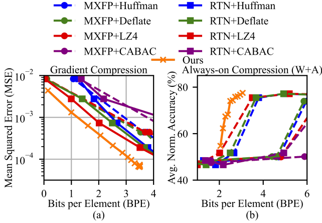
Figure 14: Information efficiency comparison with existing solutions: (a) Gradient compression MSE (lower is better) vs. average bit width. (b) Average normalized model accuracy (higher is better) across all evaluation datasets.
