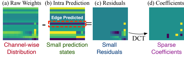
Figure 4: An example of a block of LLaMA-2-7B [78] weights going through the H.265 pipeline. The intra-prediction step generates a rough prediction of the entire block, making the residuals easy to code with the DCT transform.
