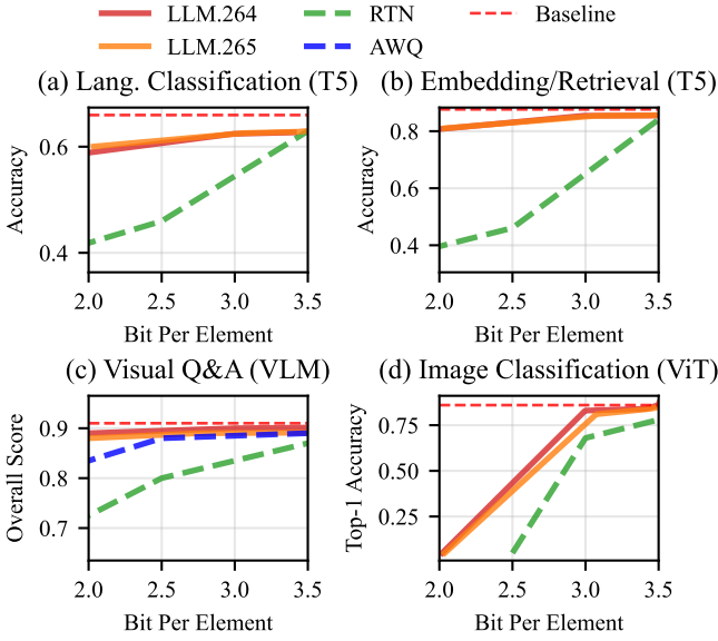
Figure 7: Evaluation of applying LLM.265 for model compression on four additional tasks: (a) Twitter Sentiment Analysis [50] using the T5 [58] model. (b) Quora Embedding/Retrieval [15] using T5 [58] model. (c) Visual Question Answering [46] using Qwen-2.5-VL-3B-Instruct model [6]. (d) ImageNet classification [18] using Vision Transformer (ViT) model [22].
