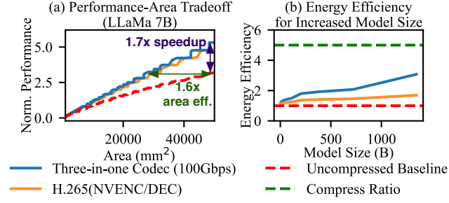
Figure 16: Impact of Communication Compression in Distributed LLM Training. The "Uncompressed Baseline" represents results without compression. The compress ratio determines the upper bound for speedup and energy efficiency.
